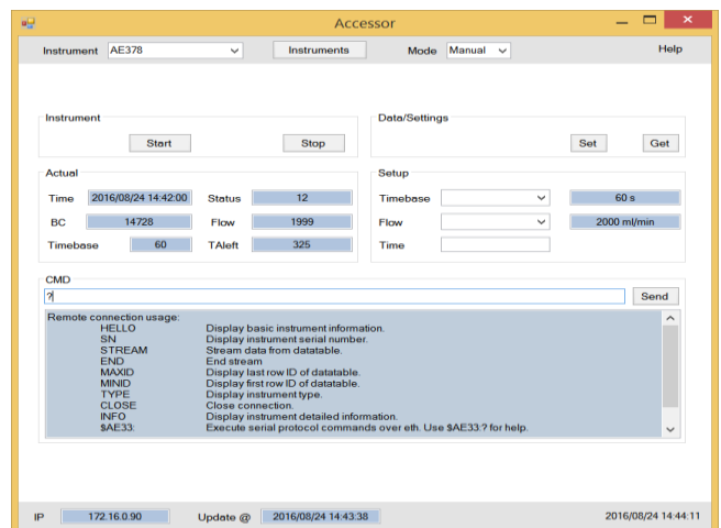
AEccessor - PC desktop application / Manual command mode
